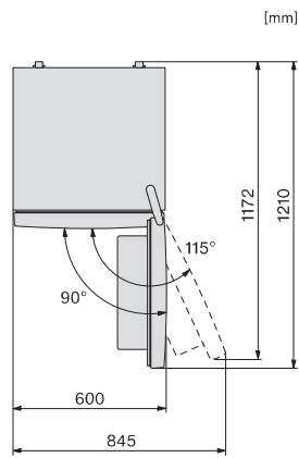
KFN4374ED, KDN4074E Active, KDN4071E Active, KDN4174E Active, KFN4391ED, KFN4394ED, top view
