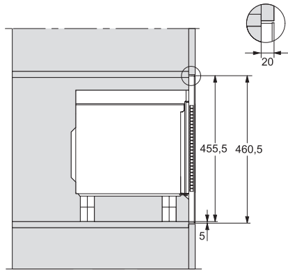
M2240SC, installation drawing
