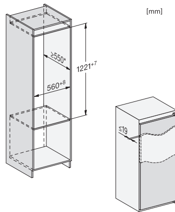
K7318D, K7328D, K7316E, K7326E, K7317D, K7327D, K7315E, K7325E, built-in
