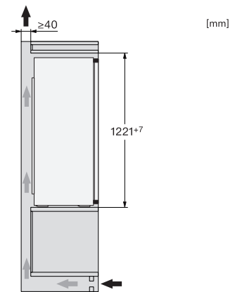
K7318D, K7328D, K7316E, K7326E, K7317D, K7327D, K7315E, K7325E, side view
