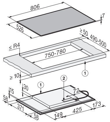
KM8482FR surface-mounted (*Fußnote) Installation drawing
